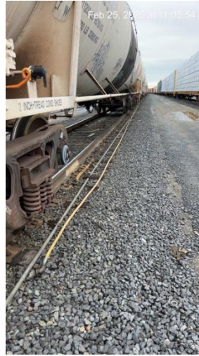
Air hose within walkway Air hose stretched out and removed from walkway
