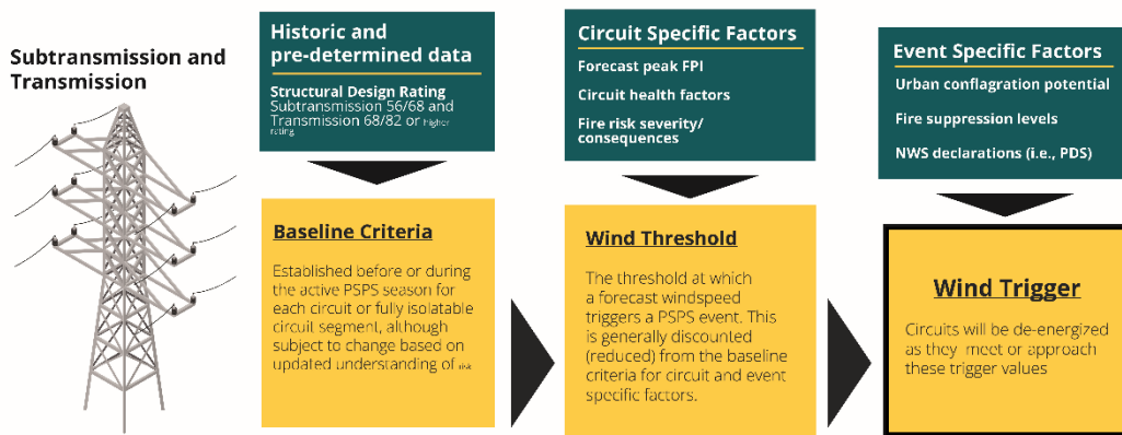
Flowchart of Decision Criteria for Subtransmission and Transmission Lines
