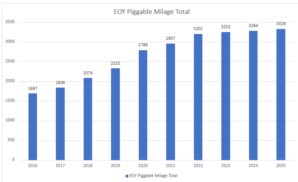
FIGURE 5-13B GAS PIPELINES THAT CAN BE INTERNALLY-INSPECTED (ANNUAL)
