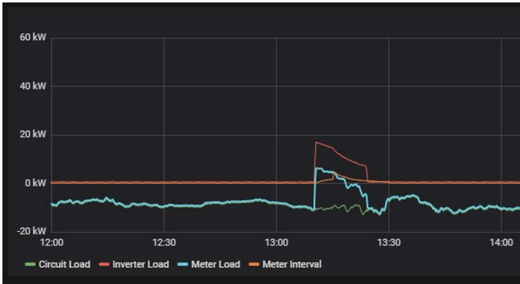
Image 3: Batteries charging with positive “Inverter Load” value.
